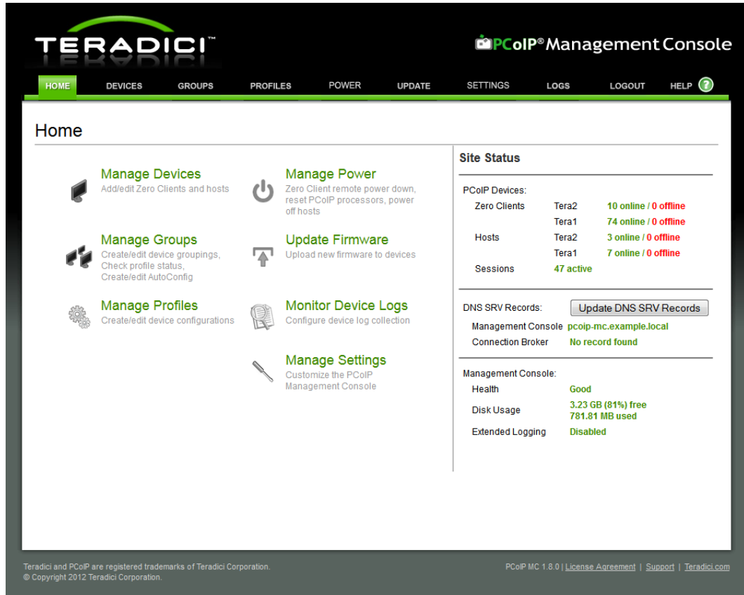
Figure 4-40: Home Webpage
